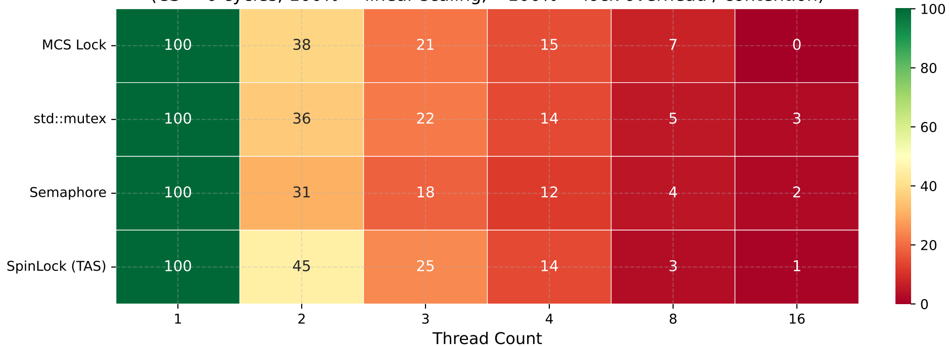
Fig 13 — Parallel Efficiency Heatmap (%) (CS = 0 cycles; 100% = linear scaling; <100% = lock overhead / contention)
